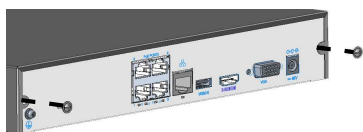
Figure 31 Rear Panel
